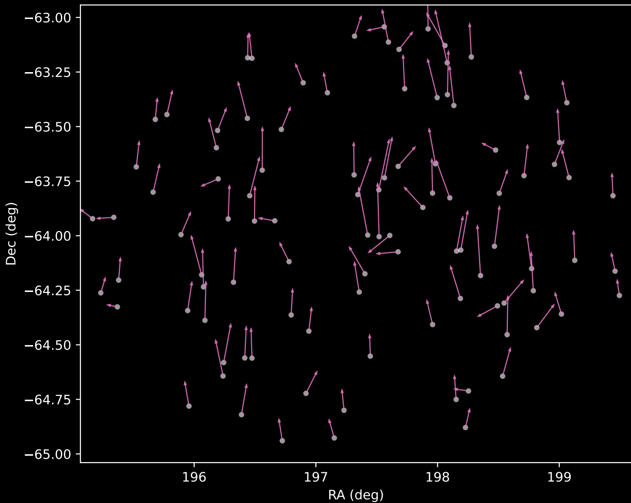
GALAH DR4 Cluster 12 Proper Motion Vectors (n=99)
