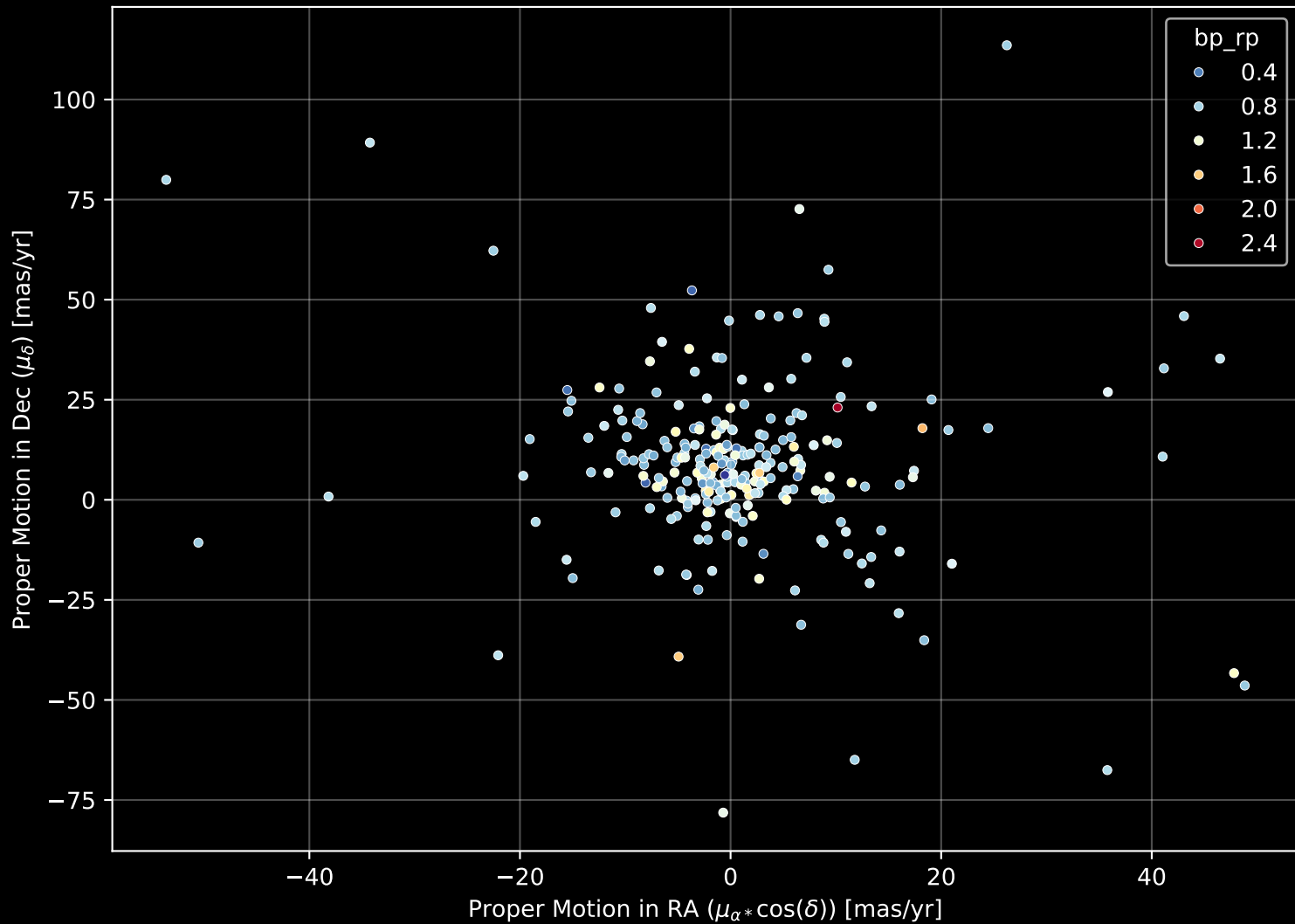
GALAH DR4 Field: [7129] Proper Motion Diagram (n= 262)
