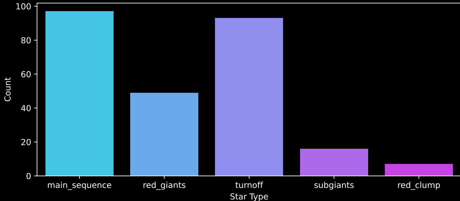
GALAH DR4 Field: [7129] Count plot of Star Type
