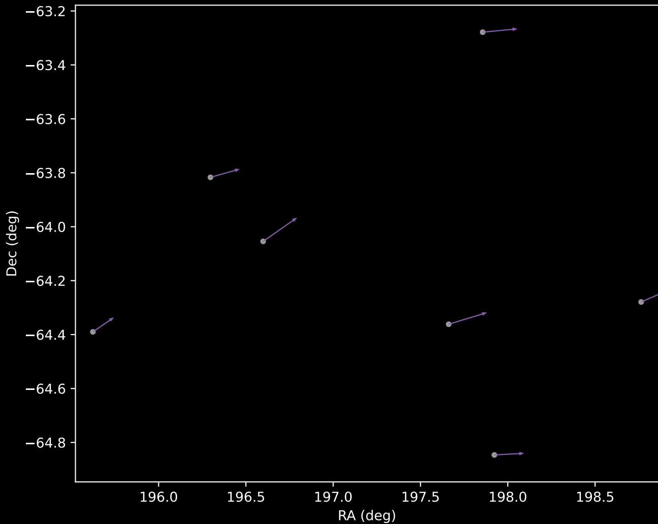
GALAH DR4 Cluster 8 Proper Motion Vectors (n=7)
