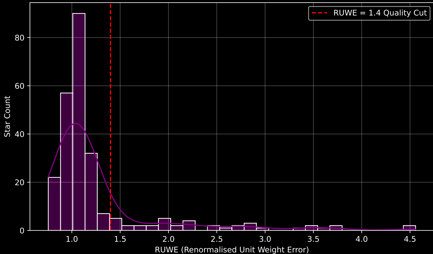
GALAH DR4 Field [7129] RUWE Distribution (n= 247)
